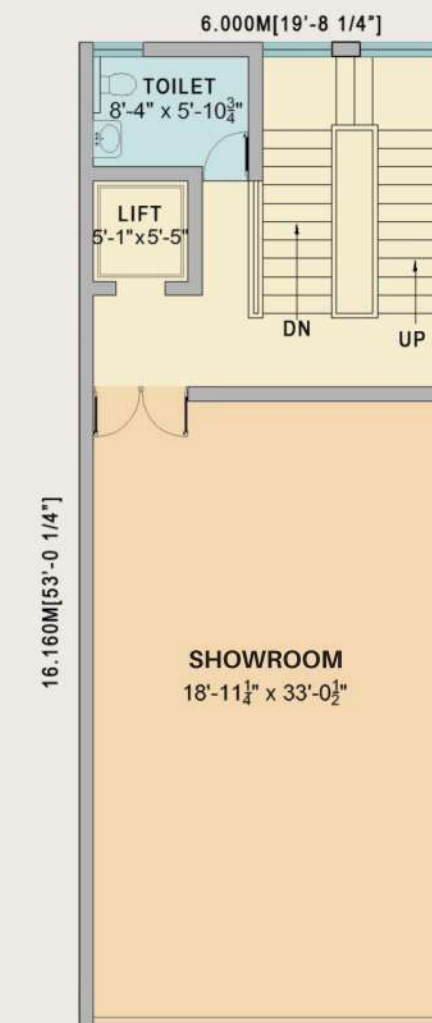
TYPICAL SECOND & THIRD FLOOR PLAN
